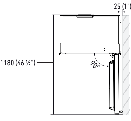
TOP VIEW, HINGE 90°
