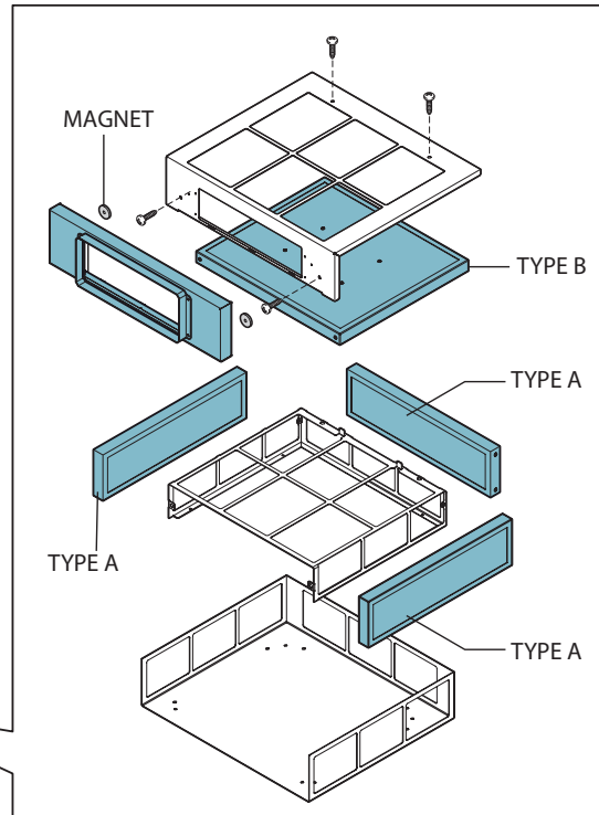
KACL. 931 (TYPE Ax3 + TYPE Bx1) RICAMBIO FILTRI - FILTER REPLACEMENT
